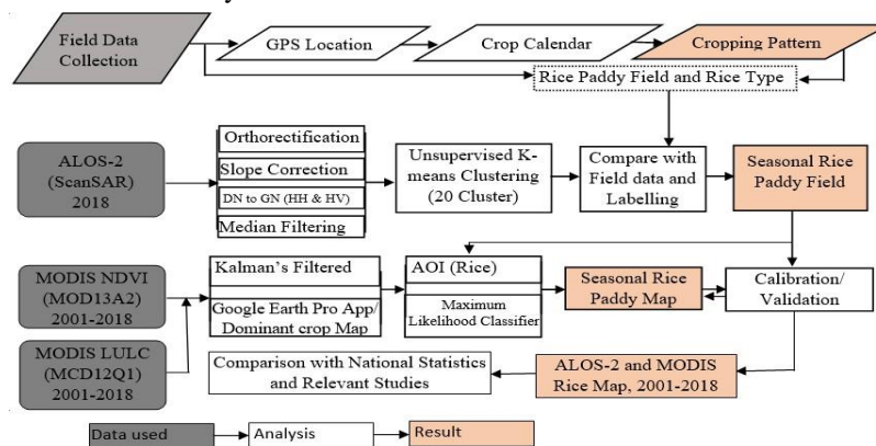
Figure 1. Overview of the rice paddy mapping framework. Geographical position system (GPS) location of rice paddy field with its cropping pattern, multi-dated PALSAR-2 HH and HV backscattered coefficient value with k-means clustering and rice are a mapping MOD13A2Kalman’s filtered NDVI data used maximum likelihood classification techniques over Bangladesh from 2001 to 2018. The flowchart illustrated the data, analysis, and result of this study
