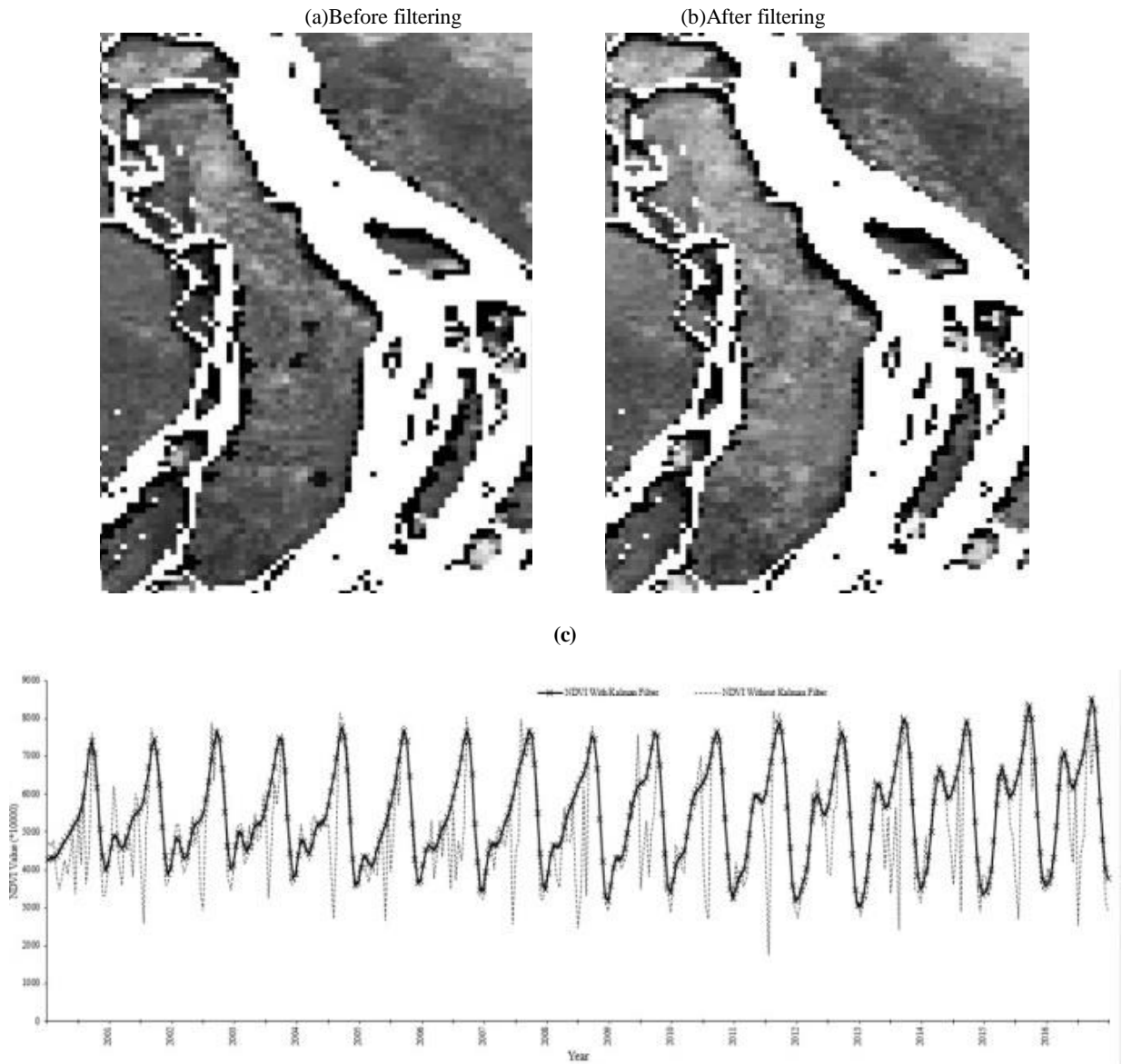
Figure 7. (a) MOD13A2 NDVI data from 2001 to 2018 before Kalman's filtered, (b) the images after filtering and (c) the temporal NDVI signature of a selected point in the study area with Kalman's filtered and without Kalman's filtered data.
