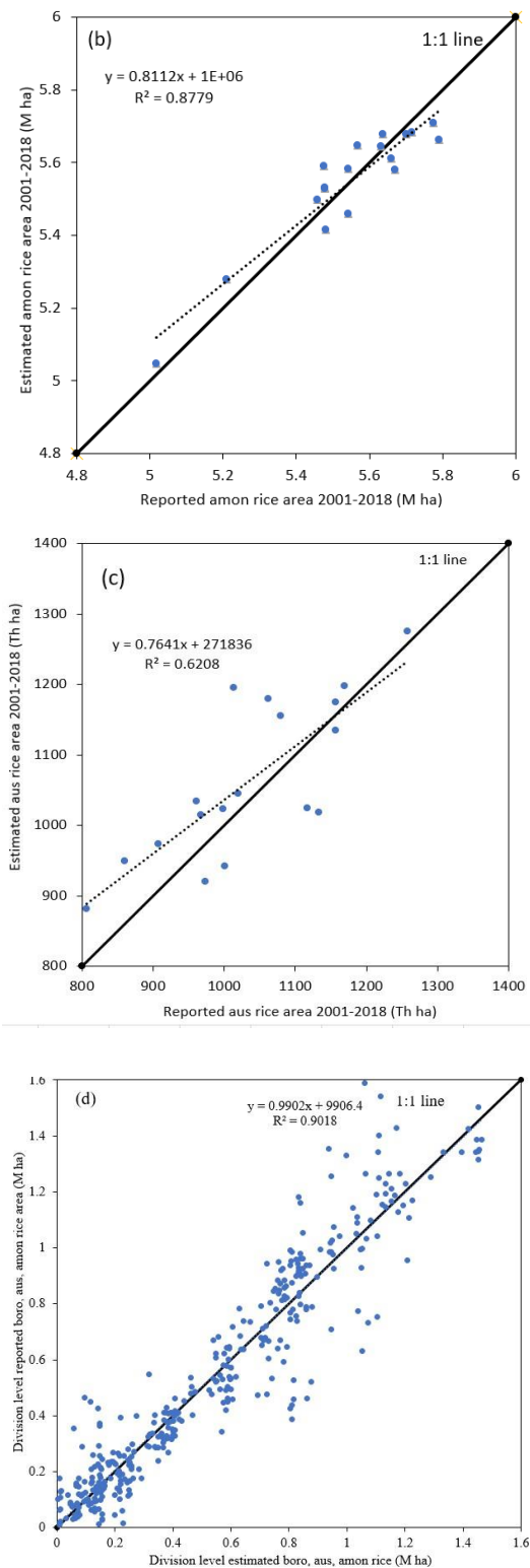
Figure 13. MODIS based rice area statistics comparison with national statistical rice area data; (a) MODIS estimated boro rice area vs national statistics reported boro rice area 2001 to
