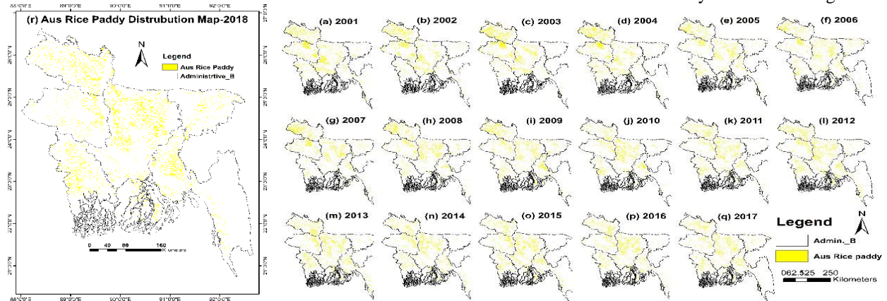
Figure 10. MODIS Kalman's filtered NDVI with maximum likelihood classifier used and ALOS-2 ScanSAR updated seasonal aus rice distribution map over the study area, (a) 2001, (b) 2002, (c) 2003, (d) 2004, (e) 2005, (f) 2006, (g) 2007, (h) 2008, (i) 2009, (j) 2010, (k) 2011, (l) 2012, (m) 2013, (n) 2014, (o) 2015, (p) 2016, (q) 2017 and (r) 2018.
