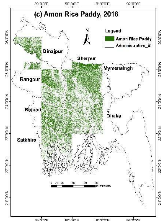
Figure 4. ALOS-2 ScanSAR backscattered coefficient unsupervised k-means class and GPS field data used seasonal rice area map overselectedtilesonBangladeshin2018, (a) Seasonal boro rice area distribution map, (b) aus rice paddy field distribution map and (c) Amon rice paddy field map.
