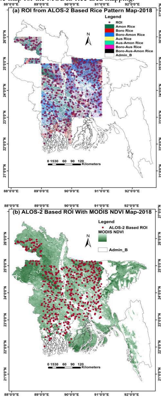
Figure 5. (a) ALOS-2 ScanSAR seasonal rice area map used region of interest (ROI) selection over the selected tiles, (b) ALOS-2 ScanSAR derived ROI used to extract the MODIS NDVI spectral value over the selected region in 2018.
