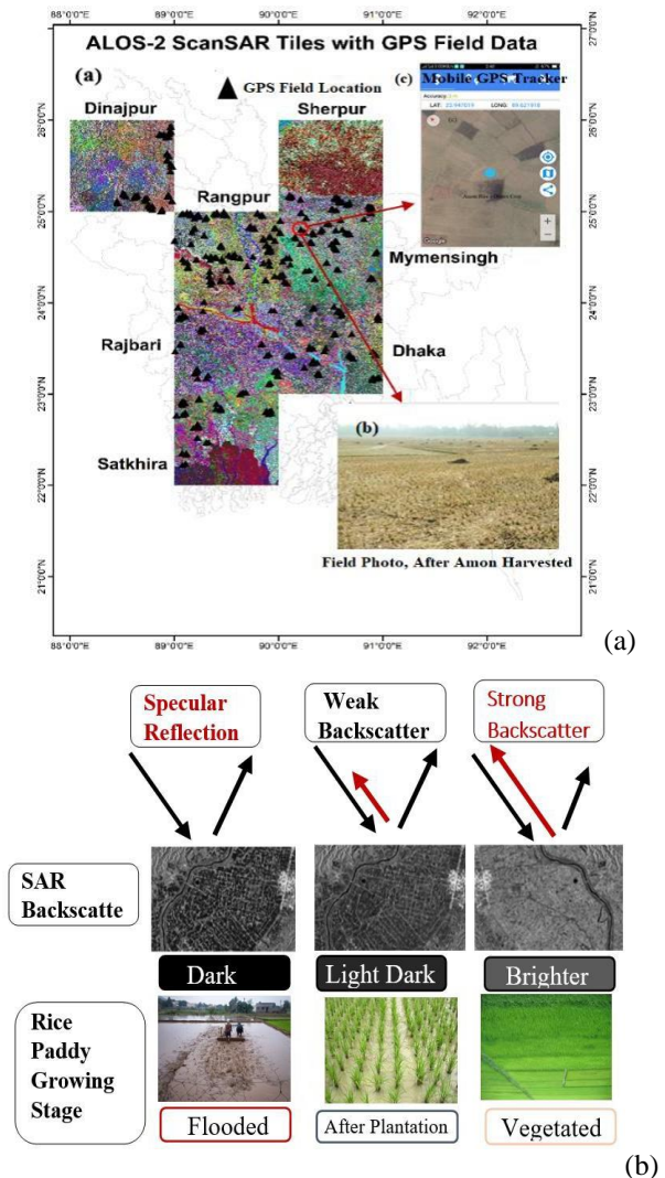
Figure 3. (a) Selected ALOS-2 ScanSAR tiles on the study area with the administrative coverage, (b) Field photo of a selected field after amon rice harvested and preparing for the boro rice plantation, (c) Mobile GPS tracker location of the field; (d) ALOS-2 ScanSAR backscattering characteristics in different rice-growing stages.
