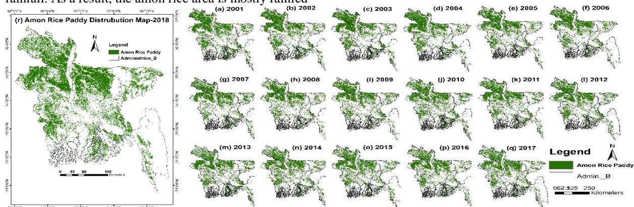
Figure 11. MODIS Kalman's filtered NDVI with maximum likelihood classifier used and ALOS-2 ScanSAR updated seasonal amon rice distribution map over the study area, (a) 2001, (b) 2002, (c) 2003, (d) 2004, (e) 2005, (f) 2006, (g) 2007, (h) 2008, (i) 2009, (j) 2010, (k) 2011, (l) 2012, (m) 2013, (n) 2014, (o) 2015, (p) 2016, (q) 2017 and (r) 2018.
