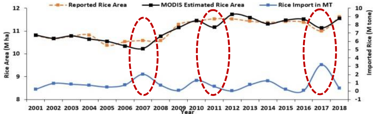
Figure 14. ALOS ScanSAR-MODIS estimated rice area compared with annual national imported rice statistics (USDA) reported from 2001 to 2018.
