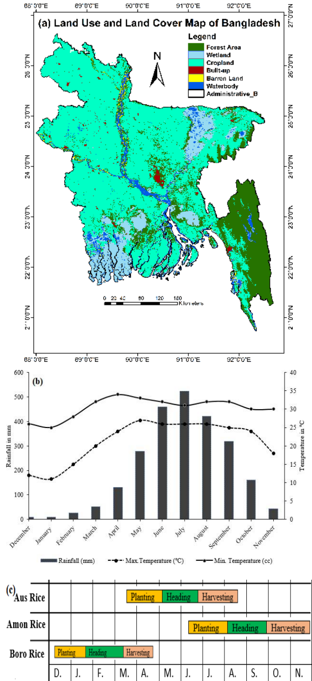
Figure 2. (a) Geographical location and generalized land use and land cover (LULC) map-207of the study area from MCD12Q1, (b) Monthly average minimum and maximum temperature, and rainfall over Bangladesh (BMD (Bangladesh Meterological Department) 2017), (c) Rice paddy crop calendar in the study area.
