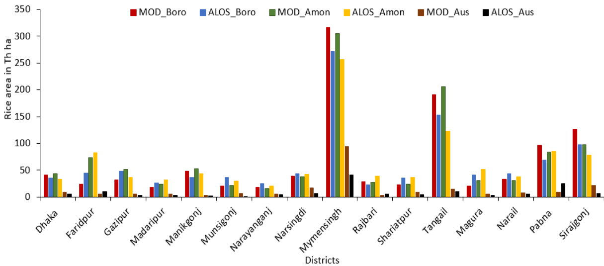
Figure 6. The ALOS-2 ScanSAR seasonal rice area statistics and MODIS rice area staistics on Boro, aus and amon rice season over the selected 16 administrative districts in 2018.
