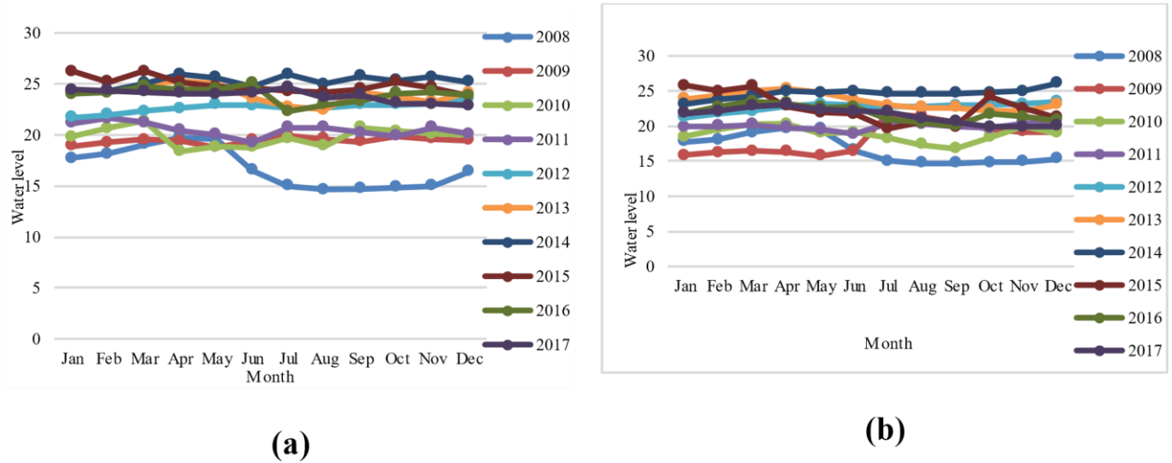
Figure 4.1: Static Groundwater level of various years at (a) Amtoli Mouza and (b) Poromanondopur Mouza in
